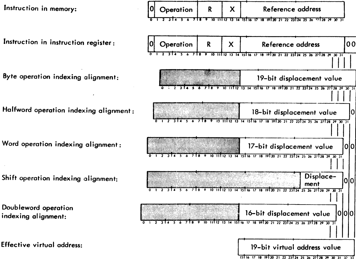
Figure 4. Index Displacement Alignment
