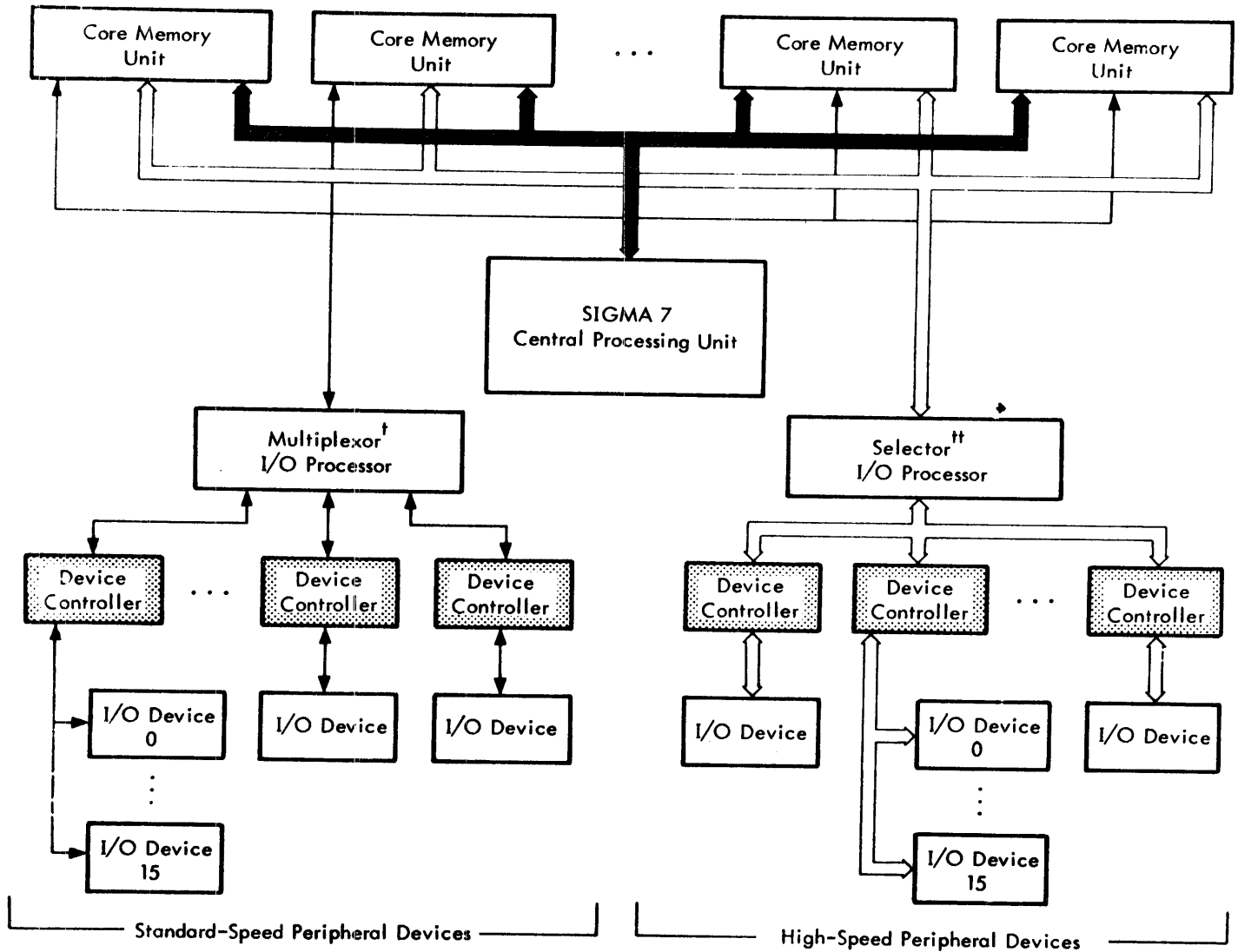
Figure 1. A Typical SIGMA 7 System
