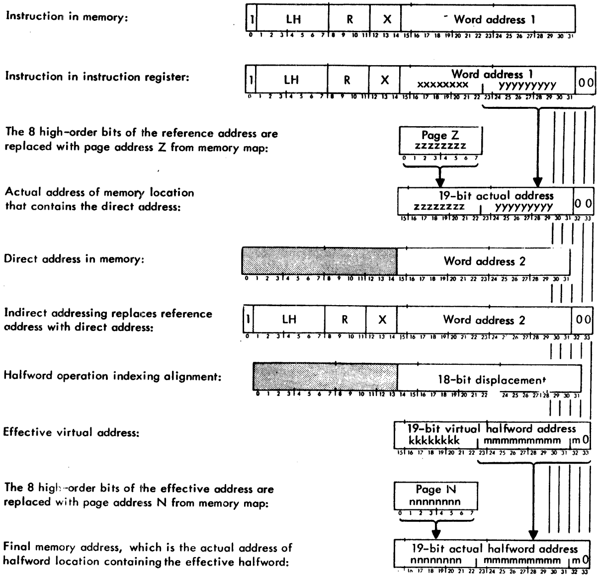
Figure 5. Generation of Actual Memory Addresses
