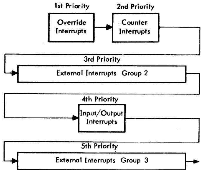
Figure 6. Typical Interrupt Priority Chain
